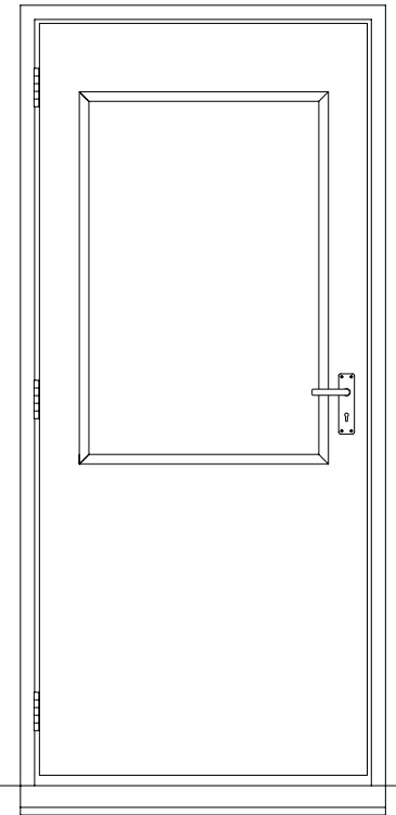
Left Hand Outward Opening - Glazed Outside View
