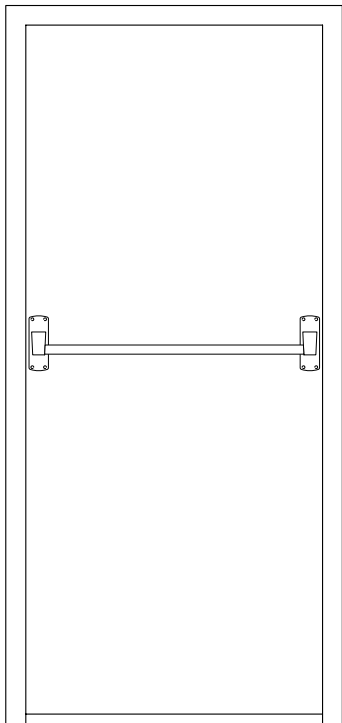
Left Hand Outward Opening - Plain Emergency Exit Inside View
