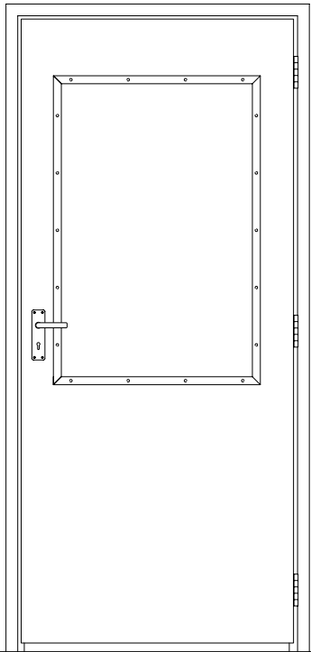
Left Hand Inward Opening - Glazed Inside View
