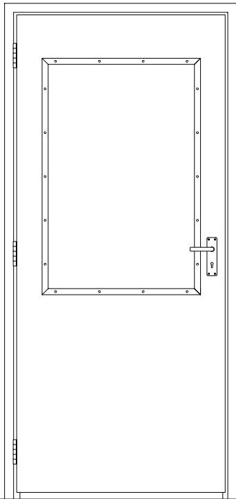
Right Hand Inward Opening - Glazed Inside View
