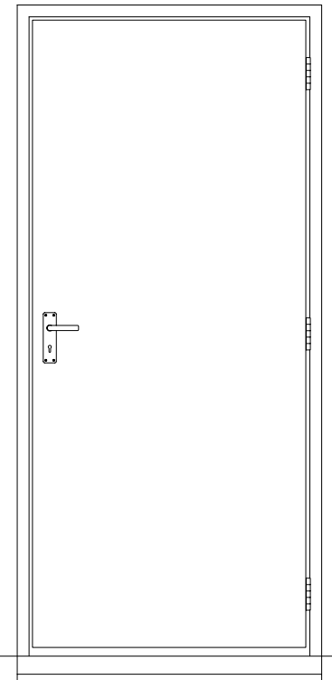
Right Hand Outward Opening - Plain Outside View
