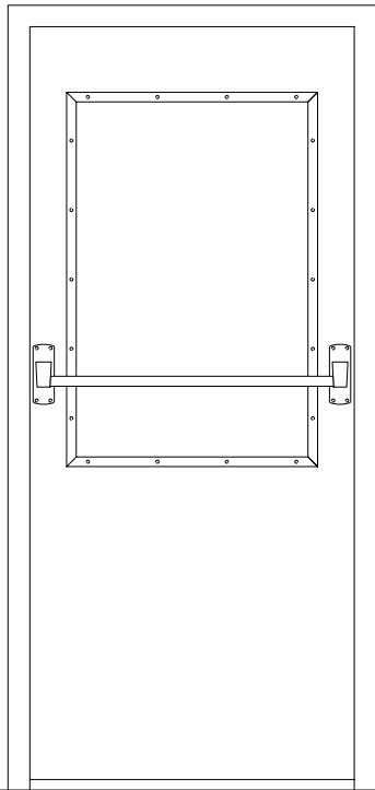
Left Hand Outward Opening - Glazed Emergency Exit Inside View
