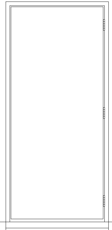
Right Hand Outward Opening - Plain Emergency Exit Outside View
